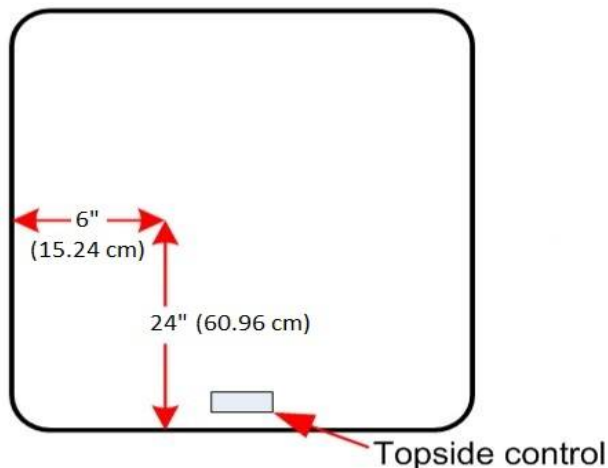
FIGURE 1: ELECTRICAL CONDUIT LOCATION
